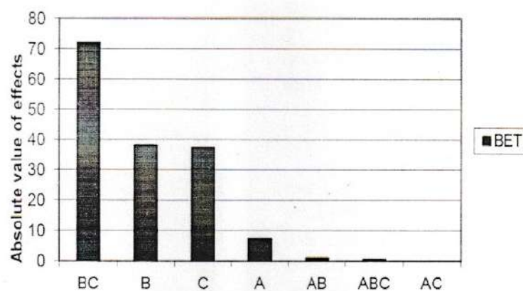
Fig. 4. Pareto plot showing the sole and interactive effects of involving parameters.
