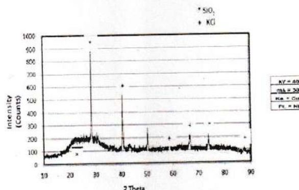
Fig. 1. Rice straw ash XRD pattern.
