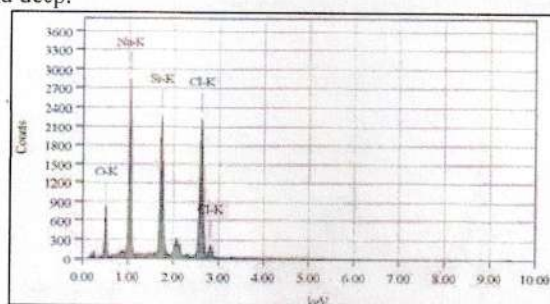
Figure 6: EDS spectrum and chemical components
