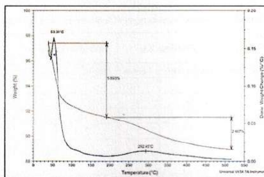
Figure 7: Thermal decomposition of silica from rice straw
