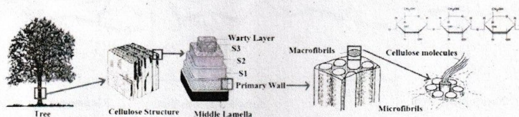
Fig. 3 Hierarchy of plant fiber
