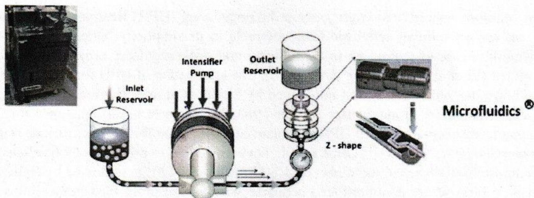
Fig. 6 Microfluidizer (Missoum et al. 2013)
