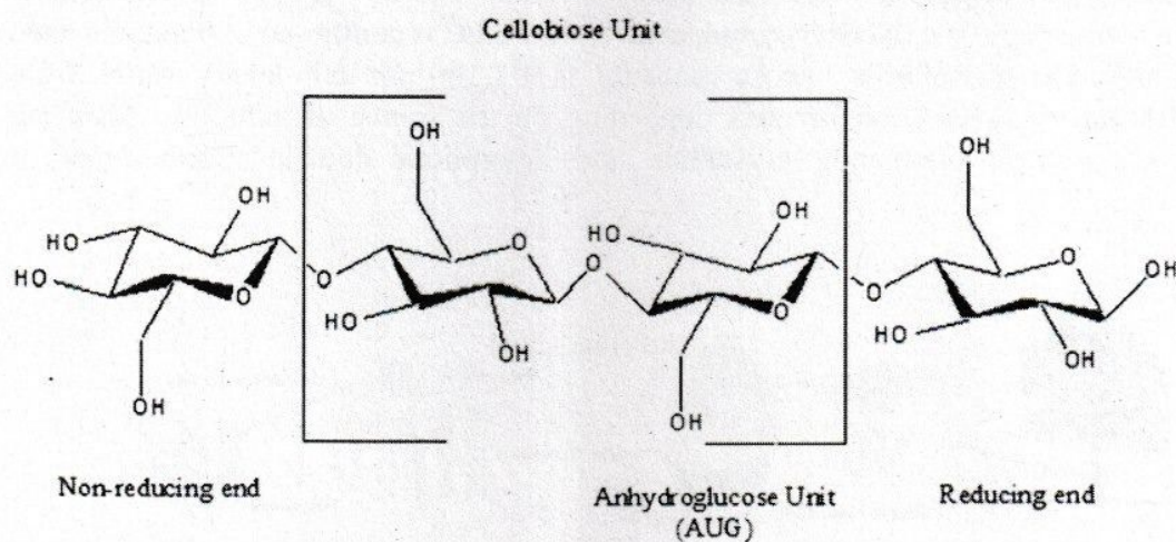
Fig. 2 The cellulose polymer chain structure
