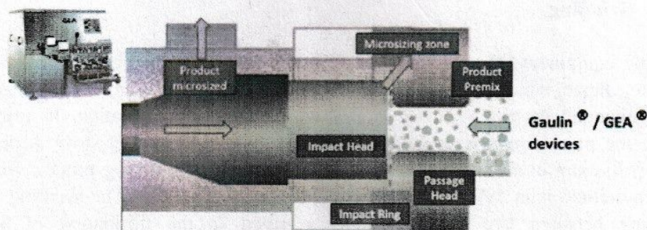
Fig. 5 High pressure homogenizer (HPH) (Missoum et al. 2013)
