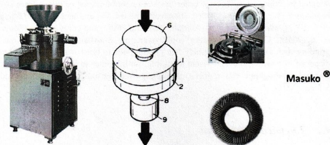
Fig. 7 Grinder (Missoum et al. 2013)
