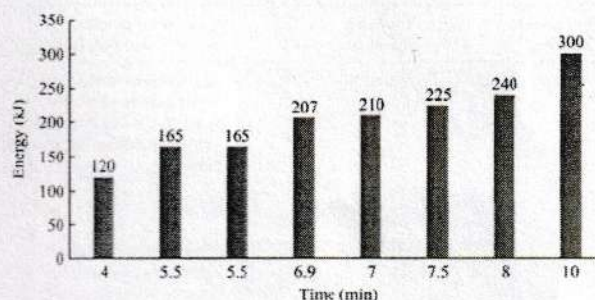
Figure 1 Relationship between processing time and consumed energy
