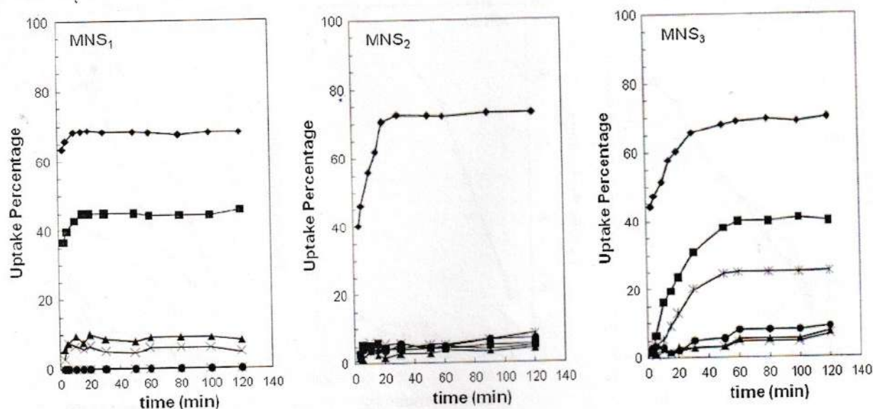
Fig. 5 Adsorption percentage of the studied metal ions (filled diamond \text{Cu}^{2+} , filled square \text{Pb}^{2+} , filled rectangle \text{Zn}^{2+} , times \text{Cd}^{2+} , asterisk \text{Co}^{2+} , filled circle \text{Ni}^{2+} ) as a function of stirring time.
