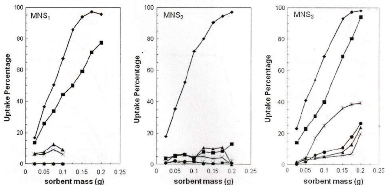
Fig. 4 Effect of amount of modified nanoparticles on adsorption efficiency of the studied metal ions (filled diamond \text{Cu}^{2+} , filled square \text{Pb}^{2+} , filled rectangle \text{Zn}^{2+} , times \text{Cd}^{2+} , asterisk \text{Co}^{2+} , filled circle
