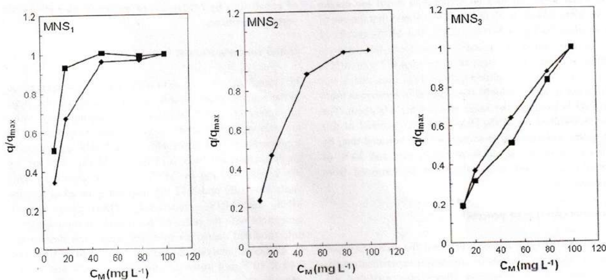
Fig. 6 Uptake of \text{Cu}^{2+} (filled diamond) and \text{Pb}^{2+} (filled square) ions by the studied adsorbents as a function of their initial concentrations in aqueous phase. Experimental conditions: adsorbent 0.15 \text{ g} , aqueous-phase pH 5, stirring time 60 \text{ min} , temperature 25^\circ \text{C}
