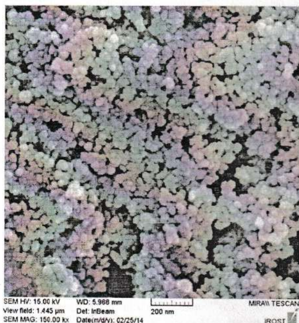
Fig. 2 SEM of the modified MNS 1
