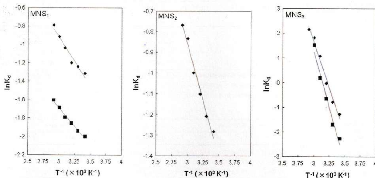
Fig. 7 Variation of \ln K_d versus T^{-1} for adsorption of \text{Cu}^{2+} (filled diamond) and \text{Pb}^{2+} (filled square) ions onto \text{MNS}_1 , \text{MNS}_2 and \text{MNS}_3 . Experimental conditions: adsorbent 0.075 g, aqueous-phase pH 5; stirring time 60 min
