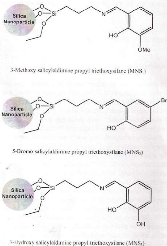
Fig. 1 Structure of the modified silica nanoparticles
