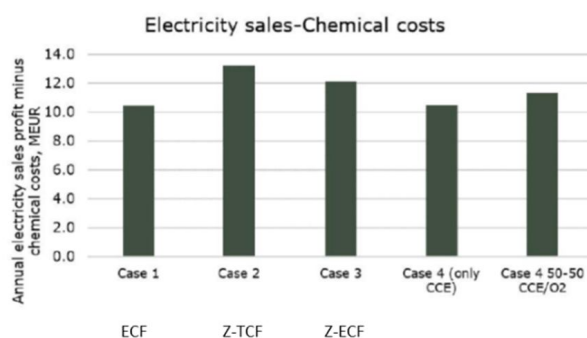
Figure 5: Annual Profits considering Electricity Sales and Bleaching Chemicals Cost [9]
