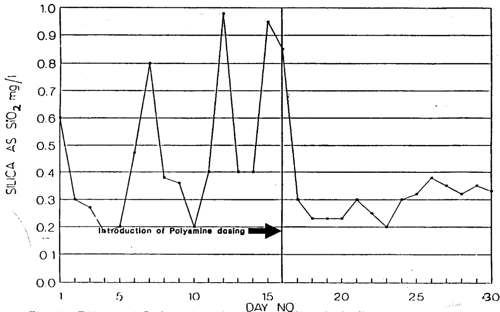
Fig 2b Effect of Polyamine dosing on Silica in boiler water
