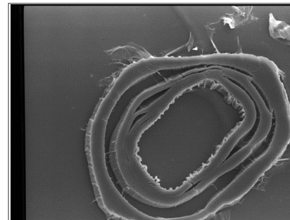
Internal De-lamination
